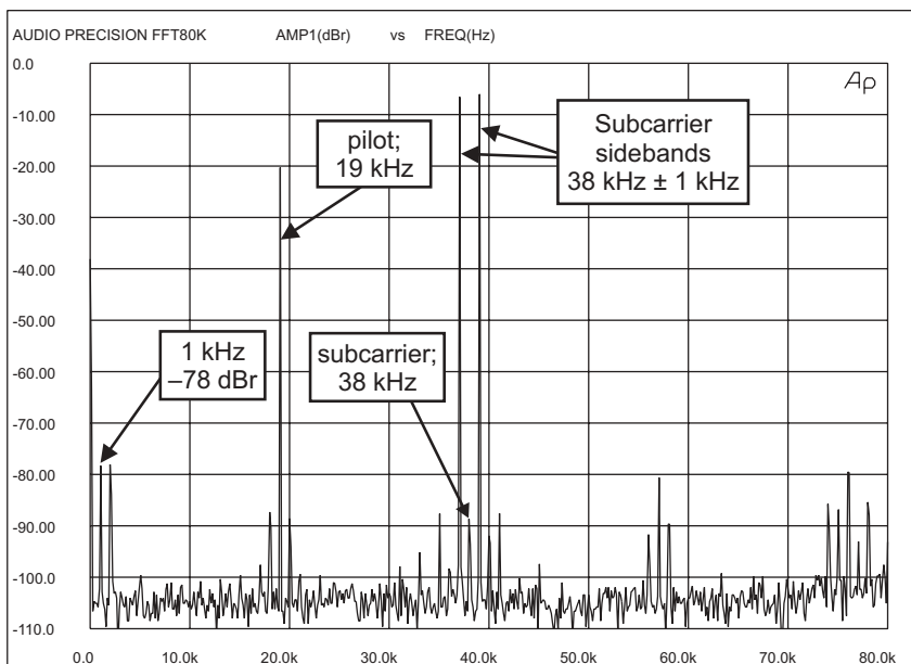
Figure 79. FFT spectrum analysis, composite FM stereo signal with 1 kHz L-R modulating signal.
