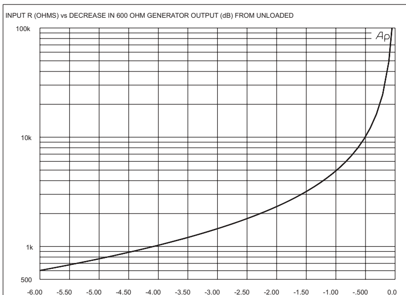
Figure 43. Input impedance vs voltage drop caused by connecting to a 600 \Omega generator, expanded at small values of voltage drop.
