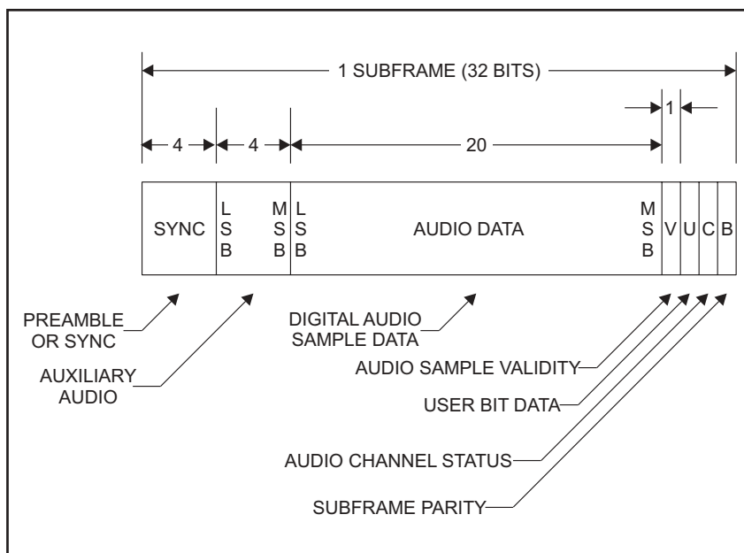
Figure 62. AES/EBU subframe structure.
