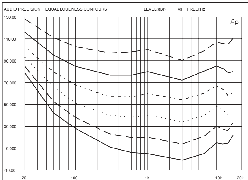
Figure 4. Fletcher-Munson curves.
