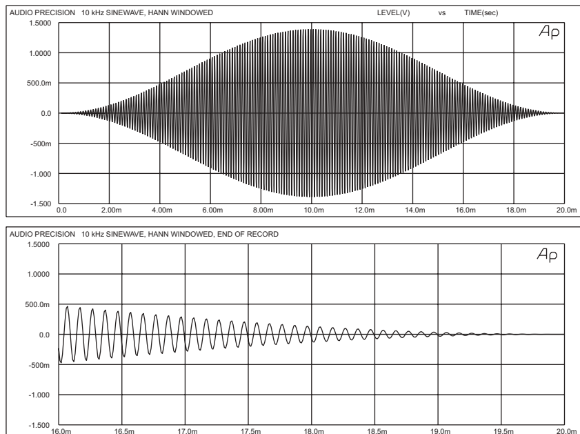
Figure 58. Continuous sine wave signal multiplied by Hann window.
