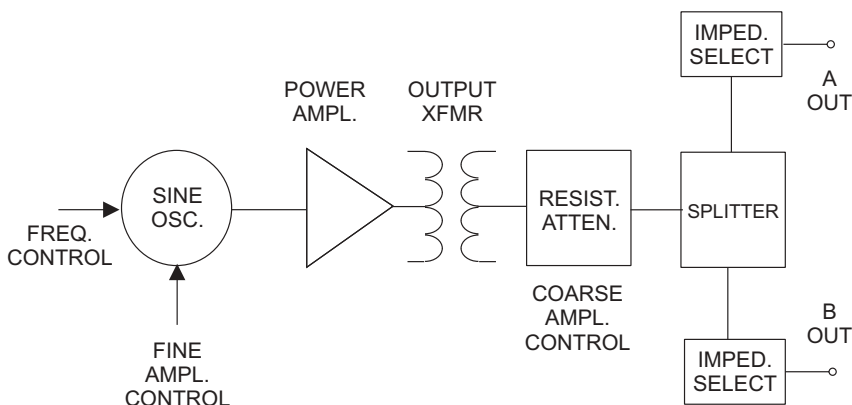
Figure 1. Block diagram, typical audio generator.
