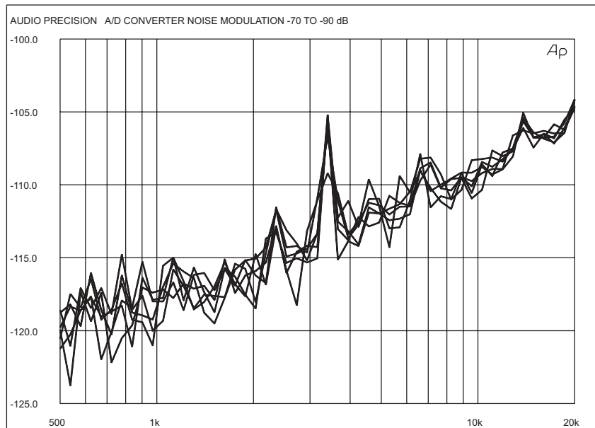
Figure 87. Noise modulation vs frequency, digital output of high-quality A/D converter at several low-signal amplitude values.
