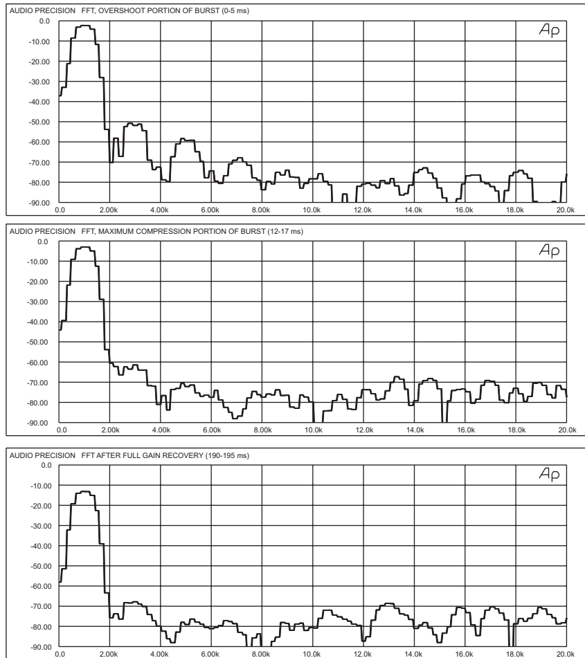
Figure 71. FFT Compressor output during attack/overshoot, steady-state compression, and gain recovery phases of burst signal in Figure 70.
