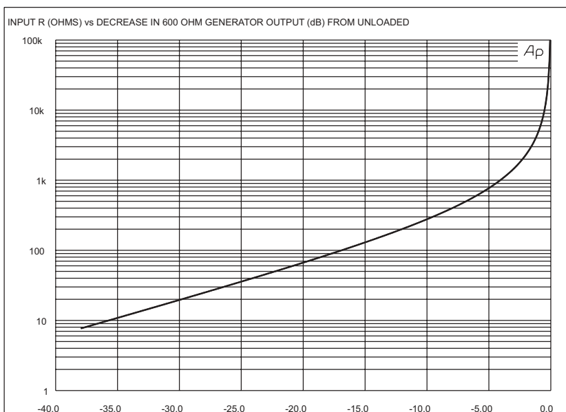
Figure 42. Input impedance vs voltage drop caused by connecting to a 600 \Omega generator.
