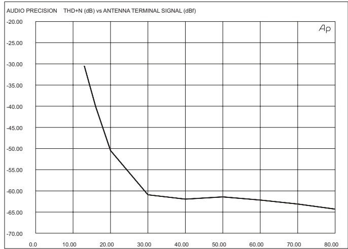
Figure 77. Typical graph of SINAD vs RF signal strength, FM receiver.
