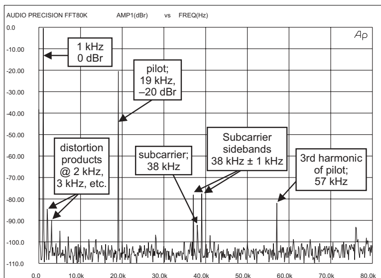
Figure 80. FFT spectrum analysis, composite FM stereo signal with 1 kHz L+R modulating signal.
